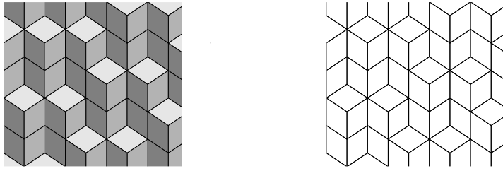
Figure 3. From a stepped plane to a tiling of the plane \Delta by three kinds of lozenges.
