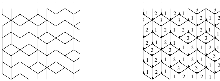
Figure 4. From a lozenge tiling of \Delta to a 2D-word.
