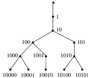
Fig. 1. The trie for the Fibonacci numeration system
