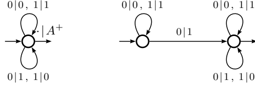
Fig. 3. A synchronized transducer for the radix order relation on A = \{0, 1\}
