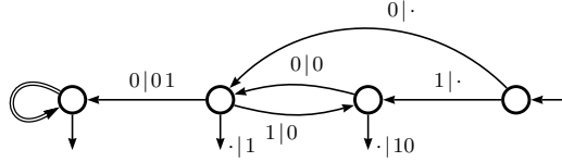
Fig. 2. The successor function for the Fibonacci numeration system
