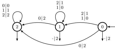
Fig. 4. The successor function for the \frac{3}{2} number system
