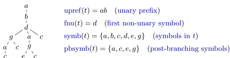
■ Figure 2 A finite tree t and its associated data.
