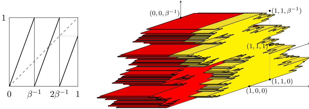
FIGURE 3. \beta -transformation and natural extension domain \mathcal{X} for \beta^2 = 2\beta + 2 .
