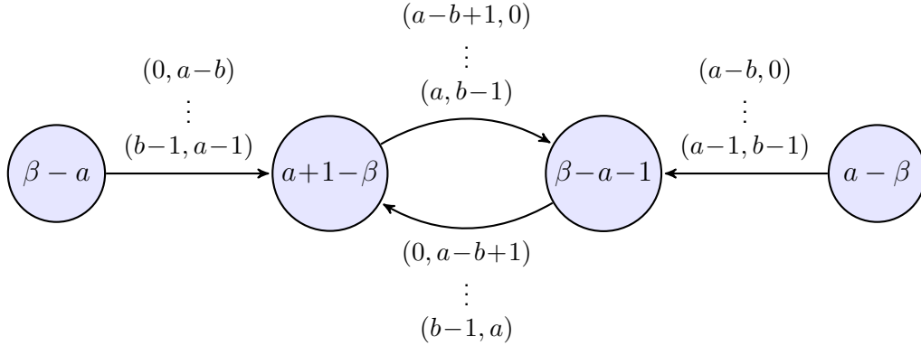
FIGURE 6. The pruned boundary graph (after merging the states with same middle component) for \beta^2 = a\beta + b , a \geq b \geq 1 .
