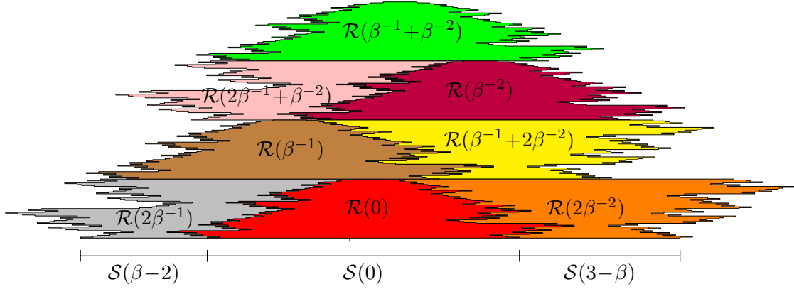
FIGURE 1. The patch \beta^{-2} \mathcal{R}(0) of the aperiodic tiling \mathcal{C}_{\text{aper}} and the corresponding integral beta-tiles, \beta^2 = 2\beta + 2 .
