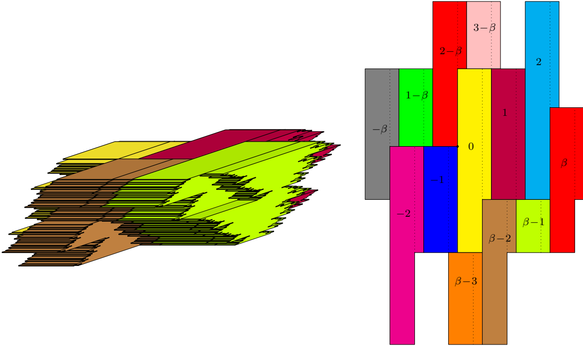
FIGURE 4. Periodic tiling \tilde{\mathcal{C}}_{\text{ext}} \subseteq \mathcal{C}_{\text{ext}} , \beta^2 = 2\beta + 2 . On the left, the following tiles are represented: \mathcal{X} (yellow), \mathcal{X} + \delta(1) (purple), \mathcal{X} + \delta(\beta - 2) (brown), \mathcal{X} + \delta(\beta - 1) (light green). On the right, the intersection with \mathbb{K}_{\infty} \times \delta_f(\{0\}) .
