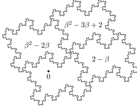
FIGURE 5. Patch of the periodic tiling \mathcal{R}(0) + \delta'(\langle \beta - 2, \beta^2 - 2\beta \rangle_{\mathbb{Z}}) induced by \beta^3 = 2\beta^2 - \beta + 1 .
