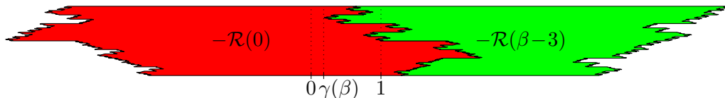
FIGURE 7. Visualization of \gamma(\beta) for \beta^2 = 3\beta + 2 .
