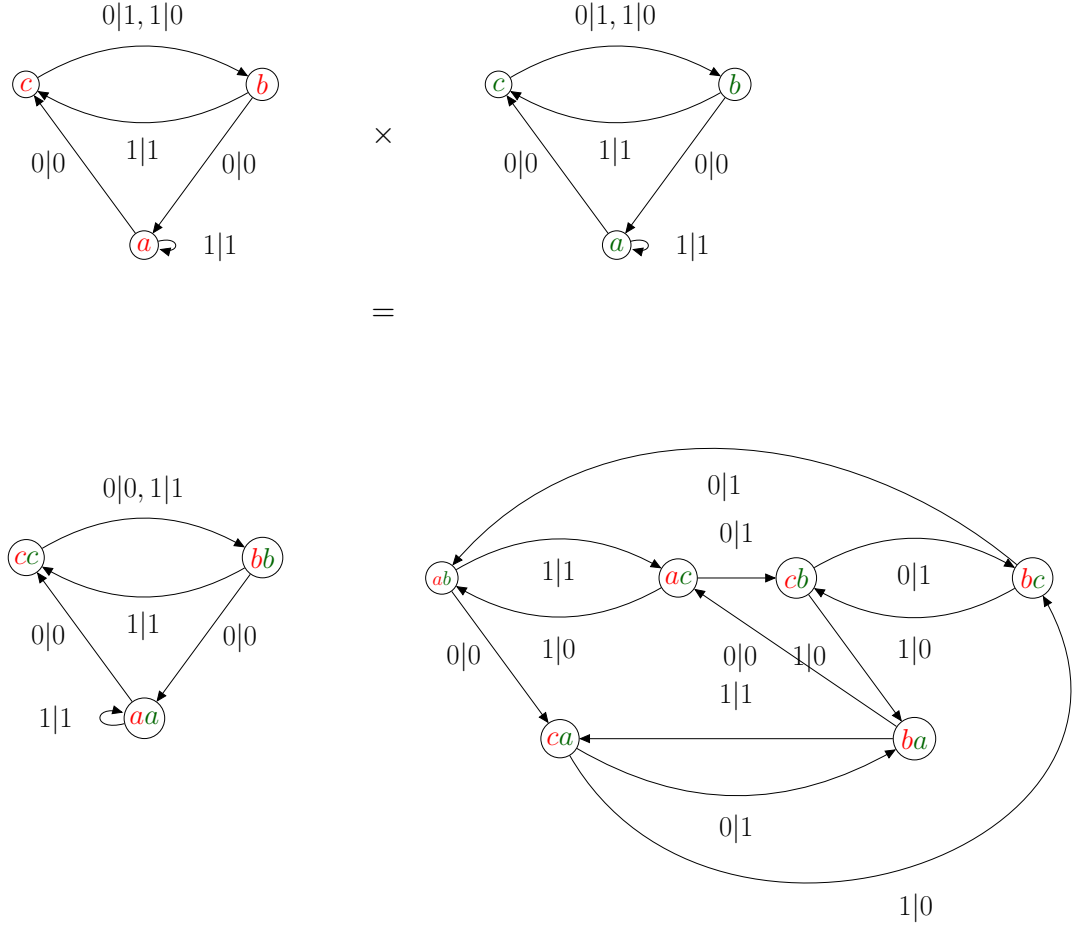
FIGURE II.1 – Le carré de l'automate Bellaterra \mathcal{B} .
