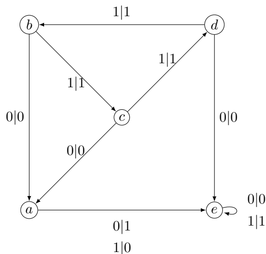
FIGURE I.23 – L'automate de Grigorchuk \mathcal{G} .
