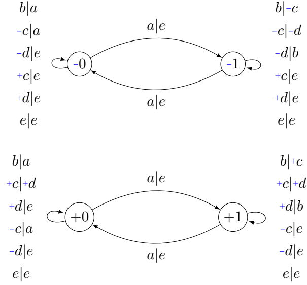
FIGURE I.3 – Le dual de l'automate Bread-and-Butterfly.
