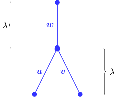
FIGURE II.10 – Tiges satisfaisant la relation u \wedge_0 v
