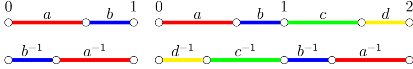
Figure 5.6: Interval exchanges U and V for the Fibonacci set and its doubling.
