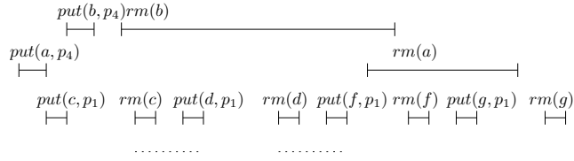
■ Figure 5 An execution that is not \text{MatchedMaxPriority}^{\text{=}} -linearizable.
