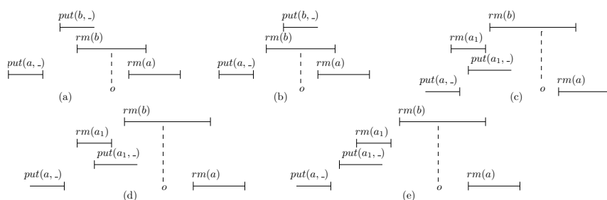
■ Figure 6 Orderings to be considered when defining a \text{MatchedMaxPriority}^{\text{=}} -complete automaton.
