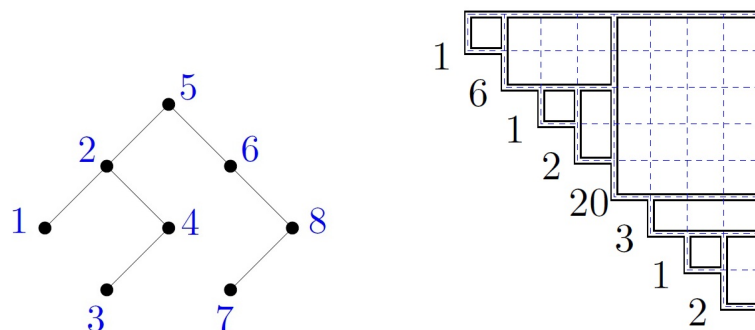
Fig. 13: A binary search labeling and a corresponding subdivision.
