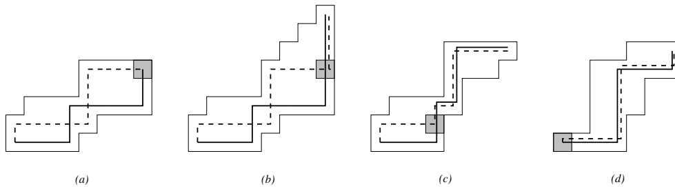
Figure 2: The paths h (solid line) and v (dashed line) in a parallelogram polyomino, where the cell C has been highlighted (a) A polyomino in \mathbb{P}_3 ; (b) A polyomino in \mathbb{P}_3^U ; (c) A polyomino in \mathbb{P}_4^R ; (d) A polyomino in \mathbb{P}_3^U where C coincides with S .
