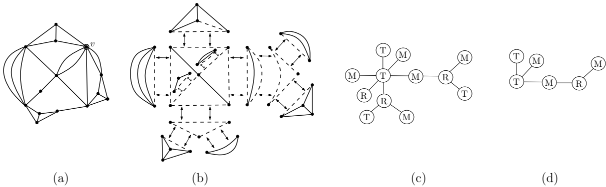
FIGURE 4. (a) A 2-connected graph. (b) The split operation. (c) Resulting brick structure (c) The associated RMT-tree. (d) The associated restricted RMT-tree if the graph is pointed at v .
