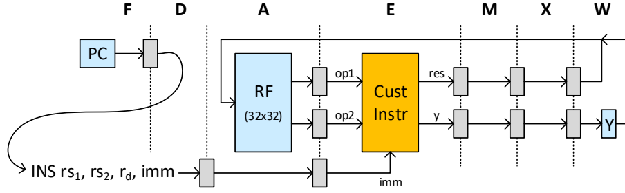
Figure 4: Integrated in the regular 7-stage pipeline as a new execution stage.
