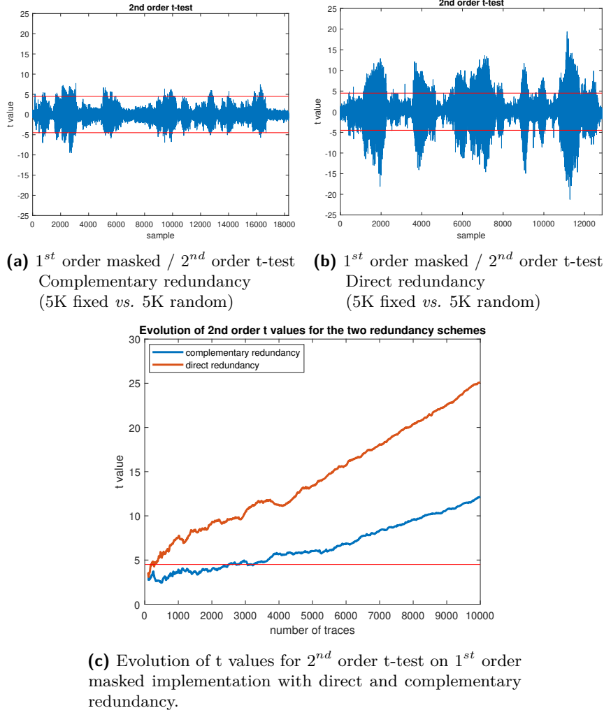
Figure 10: Effect of different redundancy schemes on power leakage.
