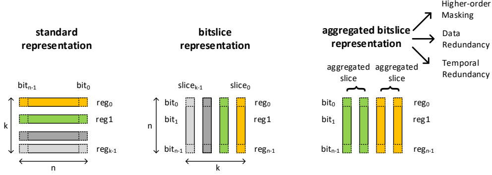
Figure 1: In a standard representation, processor registers are allocated per data word. In a bitsliced representation, processor registers are allocated per bit-weight of a block of data words. In an aggregated bitslice representation, multiple bitslices are allocated per data bit. Aggregated bitslices can be shares of a masked design, redundant data of a fault-protected design, or a combination of those.
