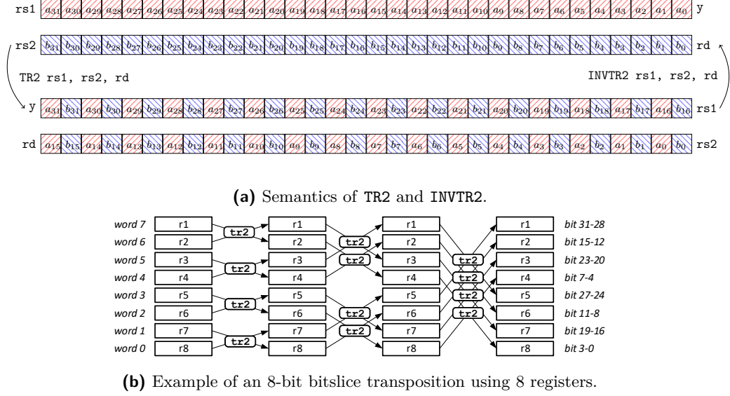
Figure 5: Transposition and its inverse
