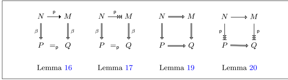
Fig. 3. Diagrams for the Lemmata Leading up to Confluence
