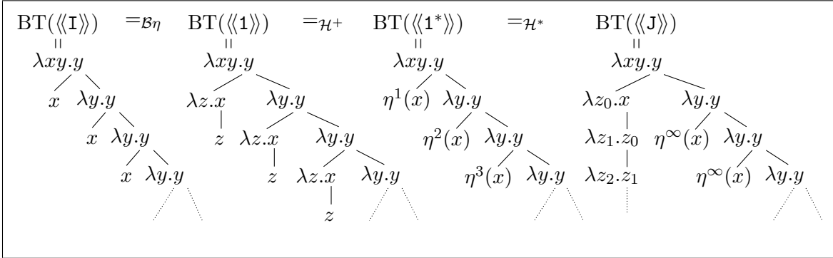
Figure 2: The Böhm trees of \langle\langle I \rangle\rangle , \langle\langle 1 \rangle\rangle , \langle\langle 1^* \rangle\rangle and \langle\langle J \rangle\rangle , where we set \eta^n(x) = BT(1^n x) and \eta^\infty(x) = BT(Jx) .
