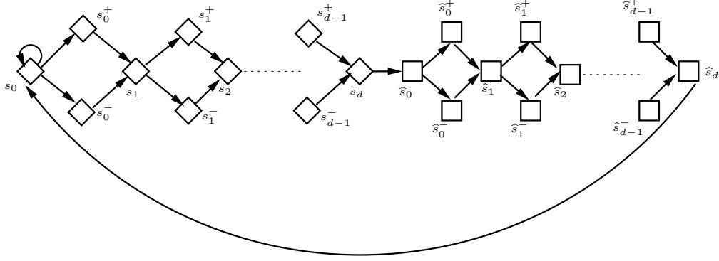
Fig. 3. Game graph for lower bound on memory.
