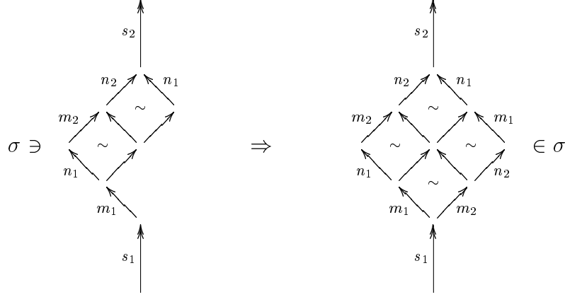
Fig. 4. Reverse consistency
