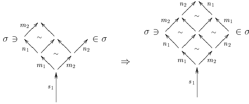
Fig. 2. Forward consistency
