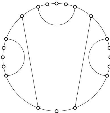
Figure 2: An outerplanar graph with \Delta = 3 and \chi^{[\#2]}(G) = 4 [36].
