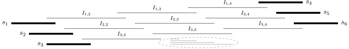
Figure 2: An interval graph of Proposition 8, reaching the order of the lower bound of Theorem 7. The construction is done for diameter D = 5 and resolving set size k = 6 . The intervals inside the dashed ellipse are the intervals that are added after the end of I_{3,2} . Similar intervals are added after the end of each interval I_{i,j} for 2 \leq j \leq 3 . The intervals \{s_1, \dots, s_6\} (in bold) form a resolving set.
