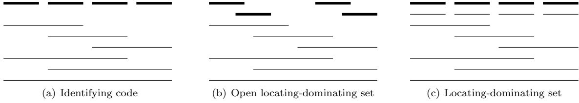
Figure 1: Examples of interval graphs from Proposition 6 reaching the lower bounds of Theorem 5. Solution intervals are in bold.
