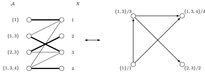
Fig. 3 Digraph of a bipartite graph
