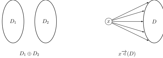
Fig. 1 Illustrations of the two operations
