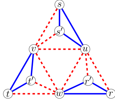
Figure 14: (G, \sigma)^*
