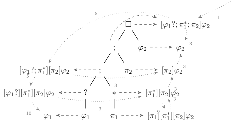
Figure 3.3: The surjection \sigma from positions in \varphi \stackrel{\text{def}}{=} [\varphi_1?; \pi_1^*; \pi_2]\varphi_2 to \text{FL}(\varphi) (dashed), and the rules used to construct \text{FL}(\varphi) (dotted).
